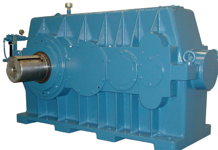
Helical and Bevel Gearboxes: D-Series
