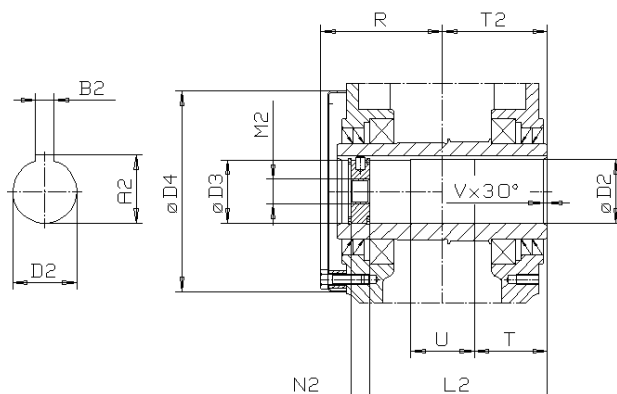
H2 Stepped shaft
