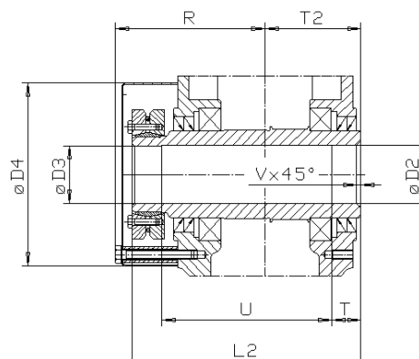
H3 Equipped with shrink disc
