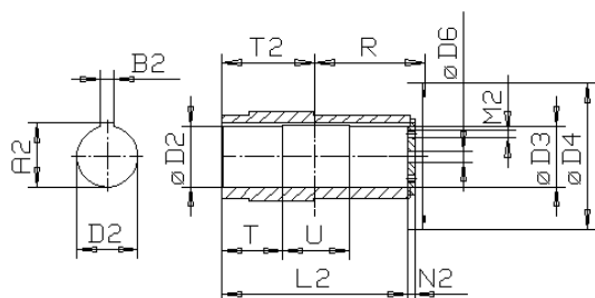
H2 Stepped shaft
